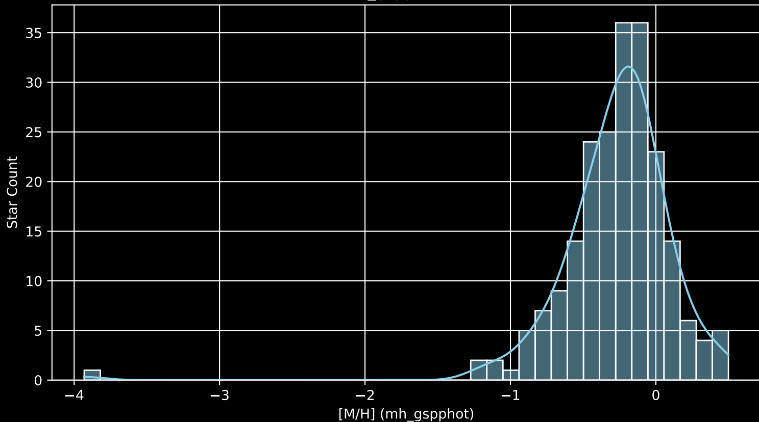
APOGEE DR17 Field: [165-30 [M/H] (mh_gspphot) (n= 214)
