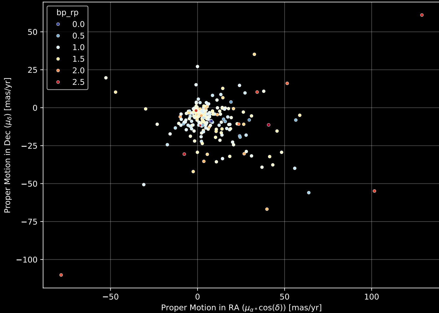
APOGEE DR17 Field: [165-30] Proper Motion Diagram (n= 215)
