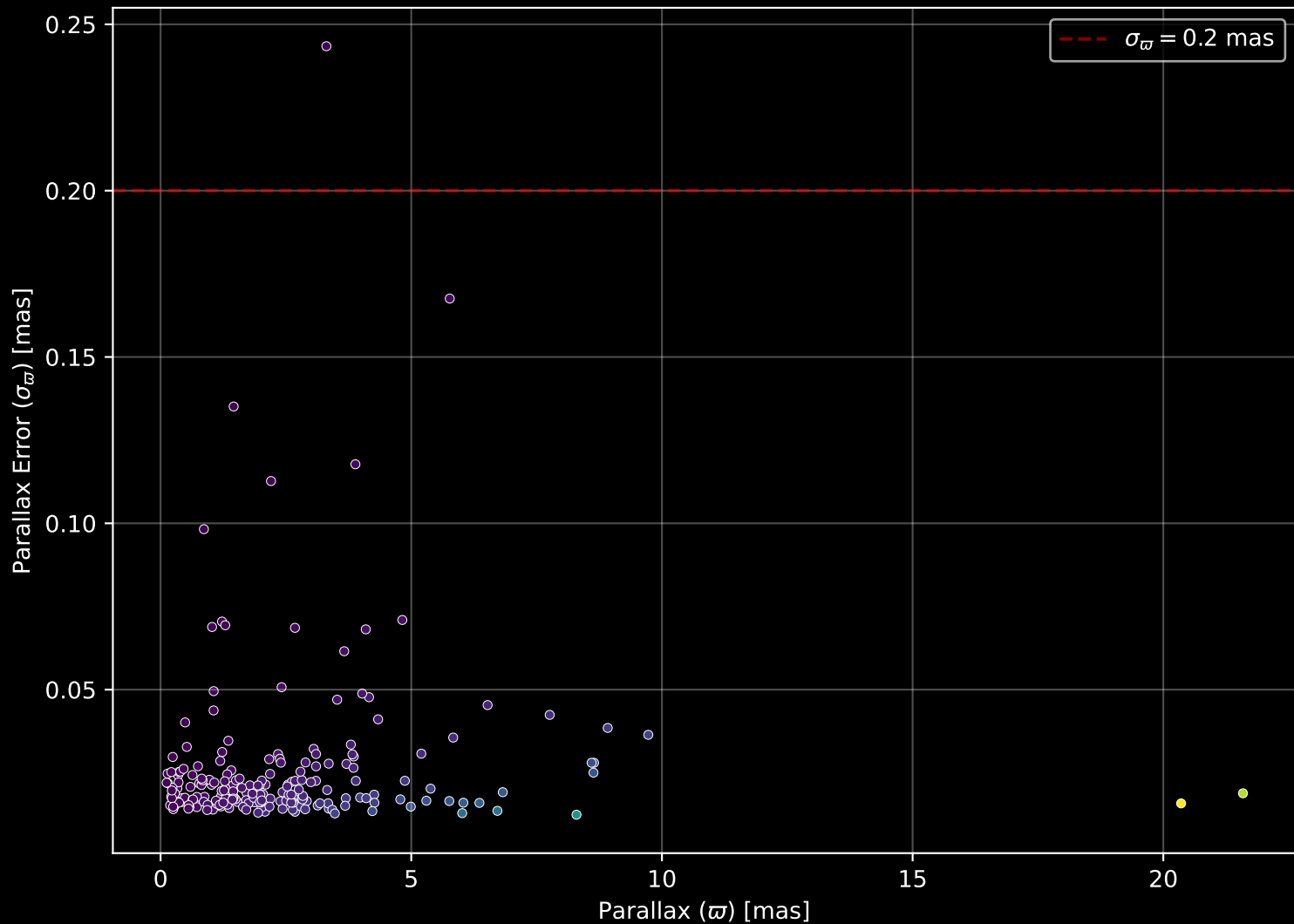
APOGEE DR17 Field: [165-30] Parallax Quality (n= 215)
