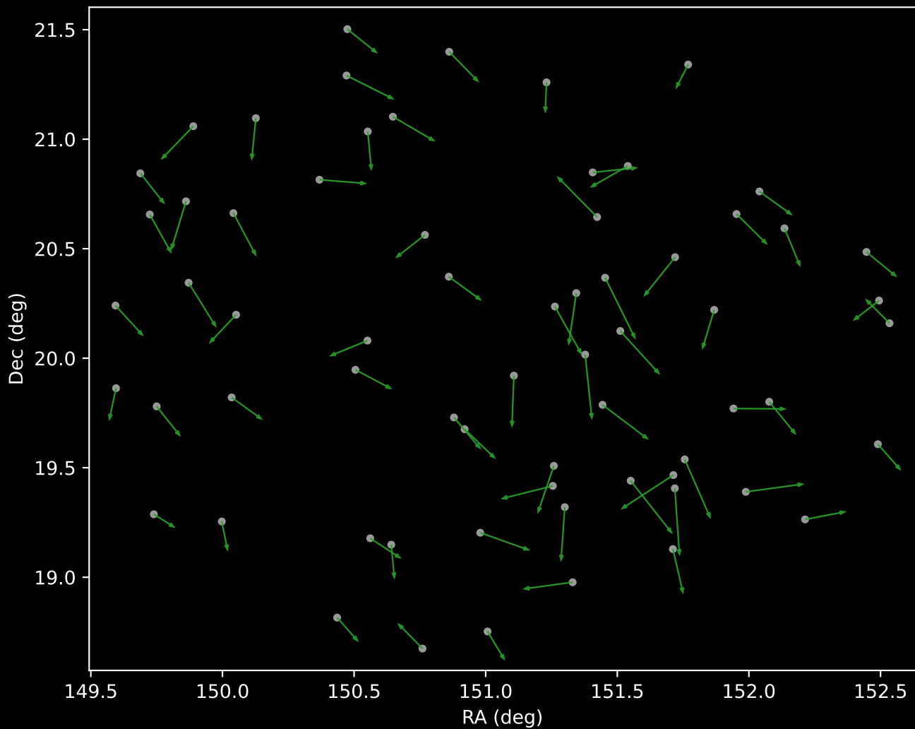
APOGEE DR17 Cluster 4 Proper Motion Vectors (n=66)
