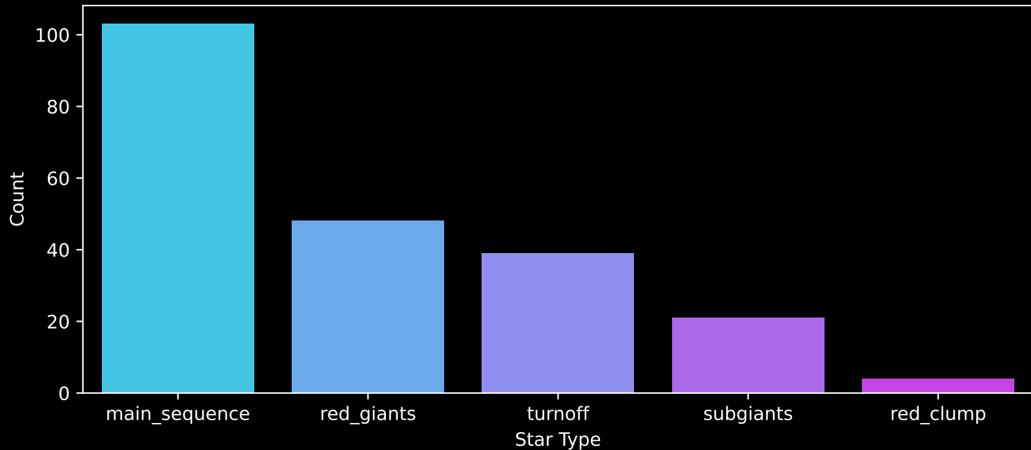
APOGEE DR17 Field: [165-30] Count plot of Star Type
