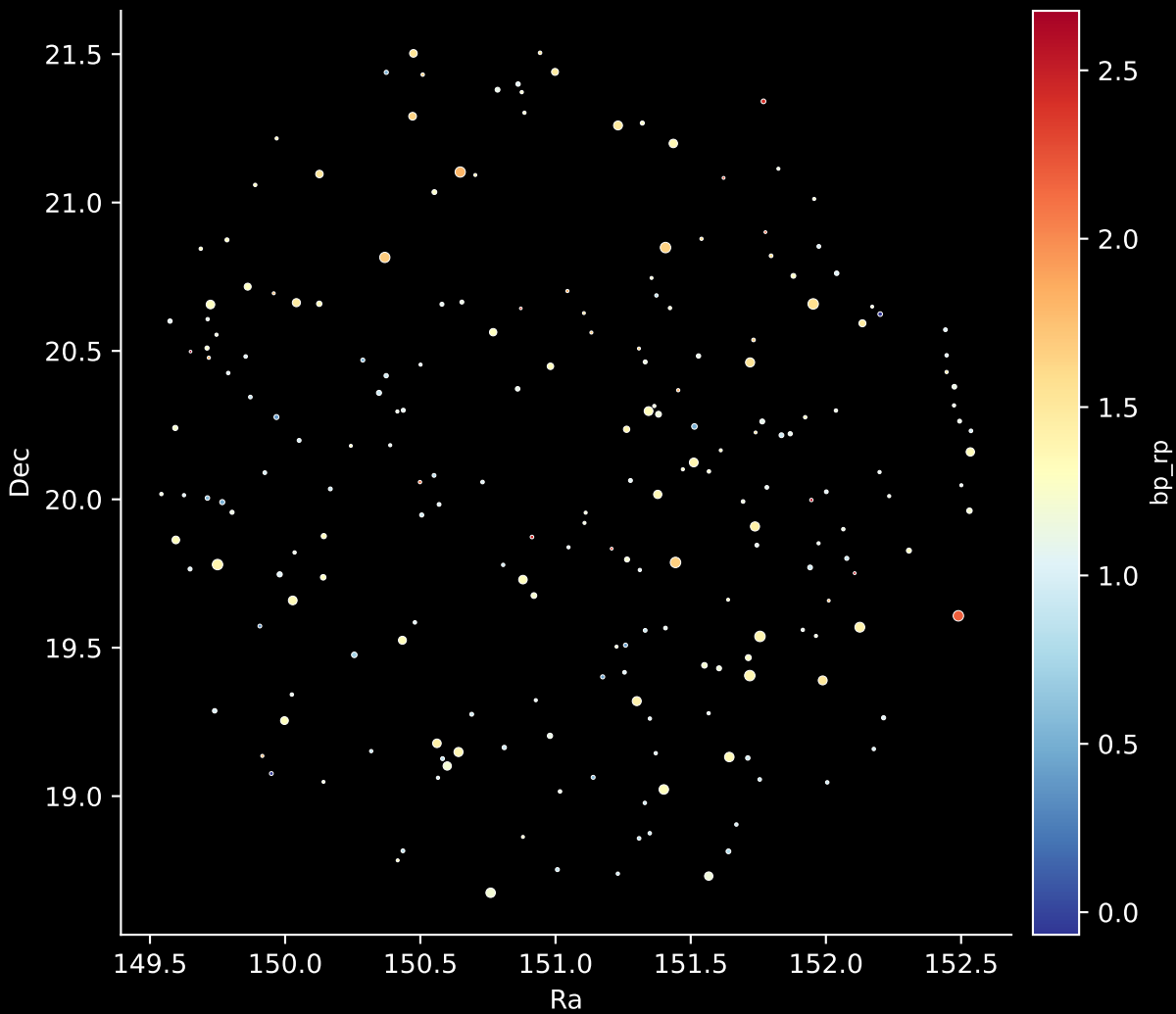
APOGEE DR17 Field: [165-30] Stars: 215
