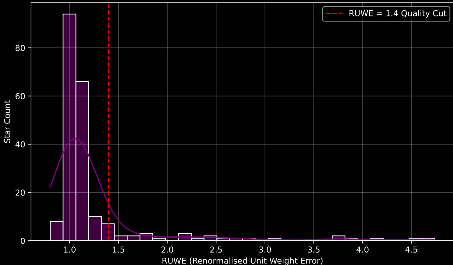
GAPOGEE DR17 Field [165-30] RUWE Distribution (n= 209)
