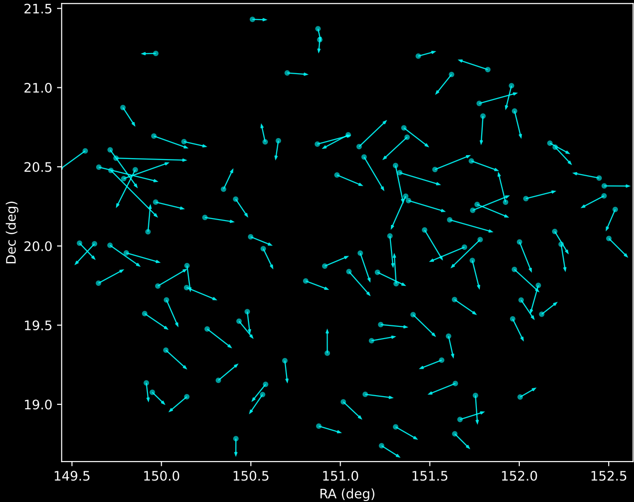
APOGEE DR17 Noise Stream Proper Motion Vectors (n=114)
